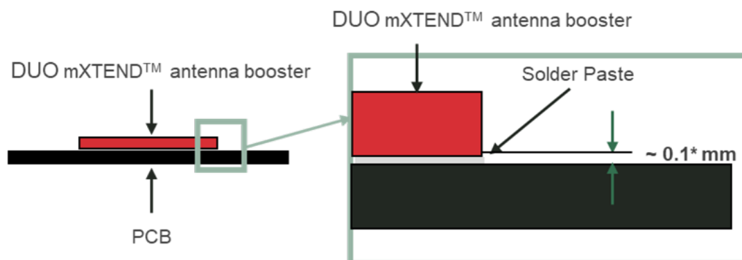
Figure 19 – Soldering Details.
