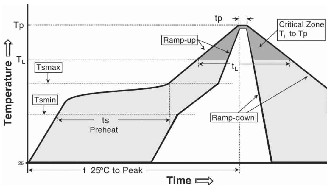
Figure 20 – Temperature profile.
